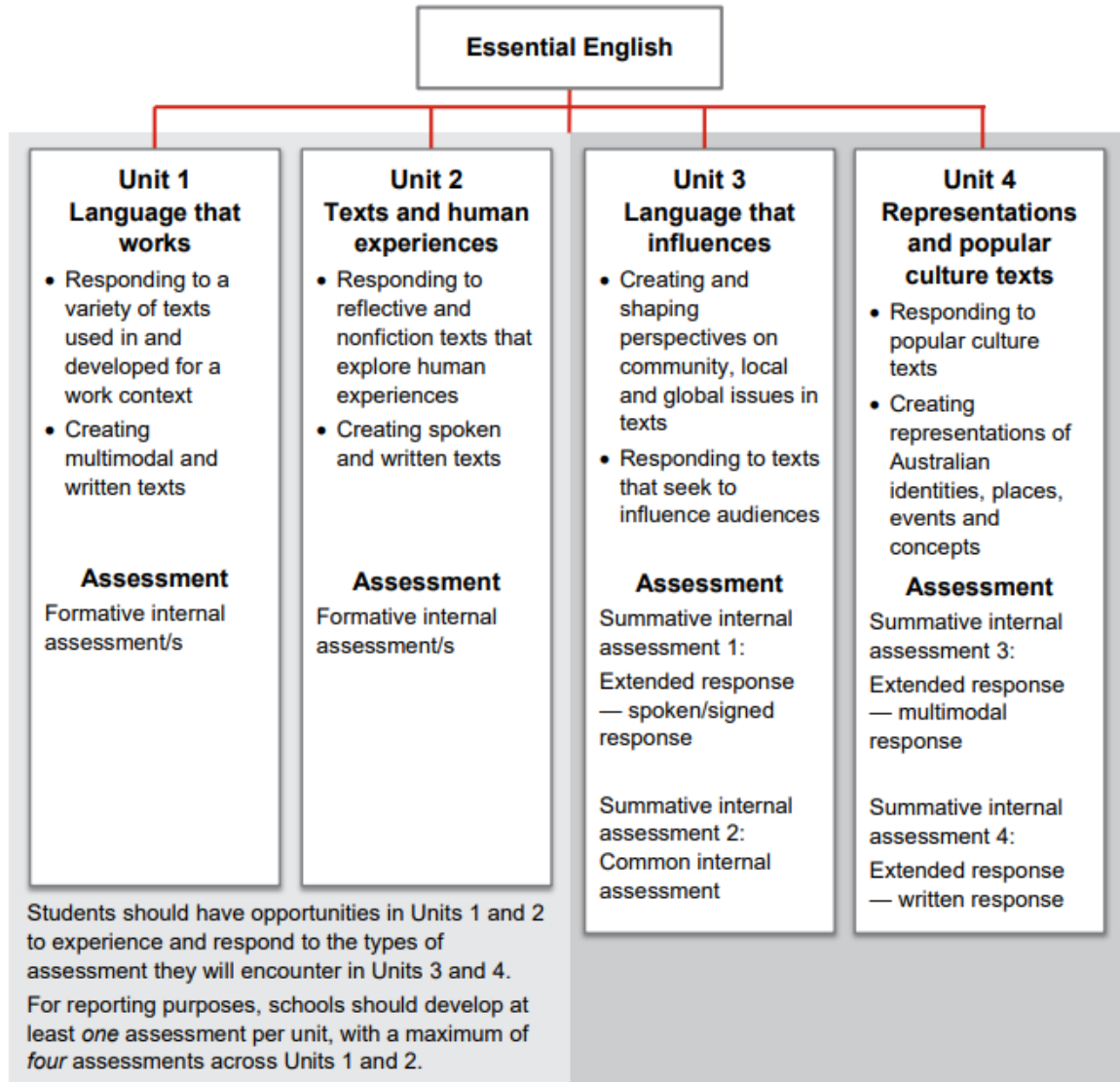
Figure 2: Course structure
