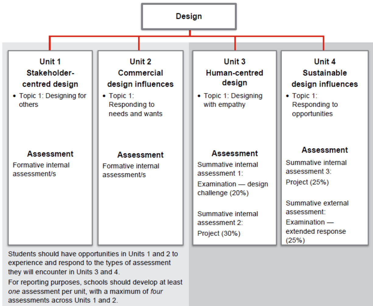
Figure 2: Course structure
