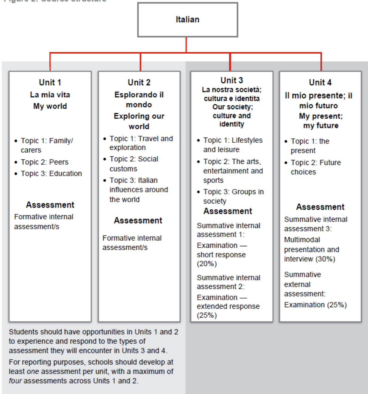
Figure 2: Course structure
