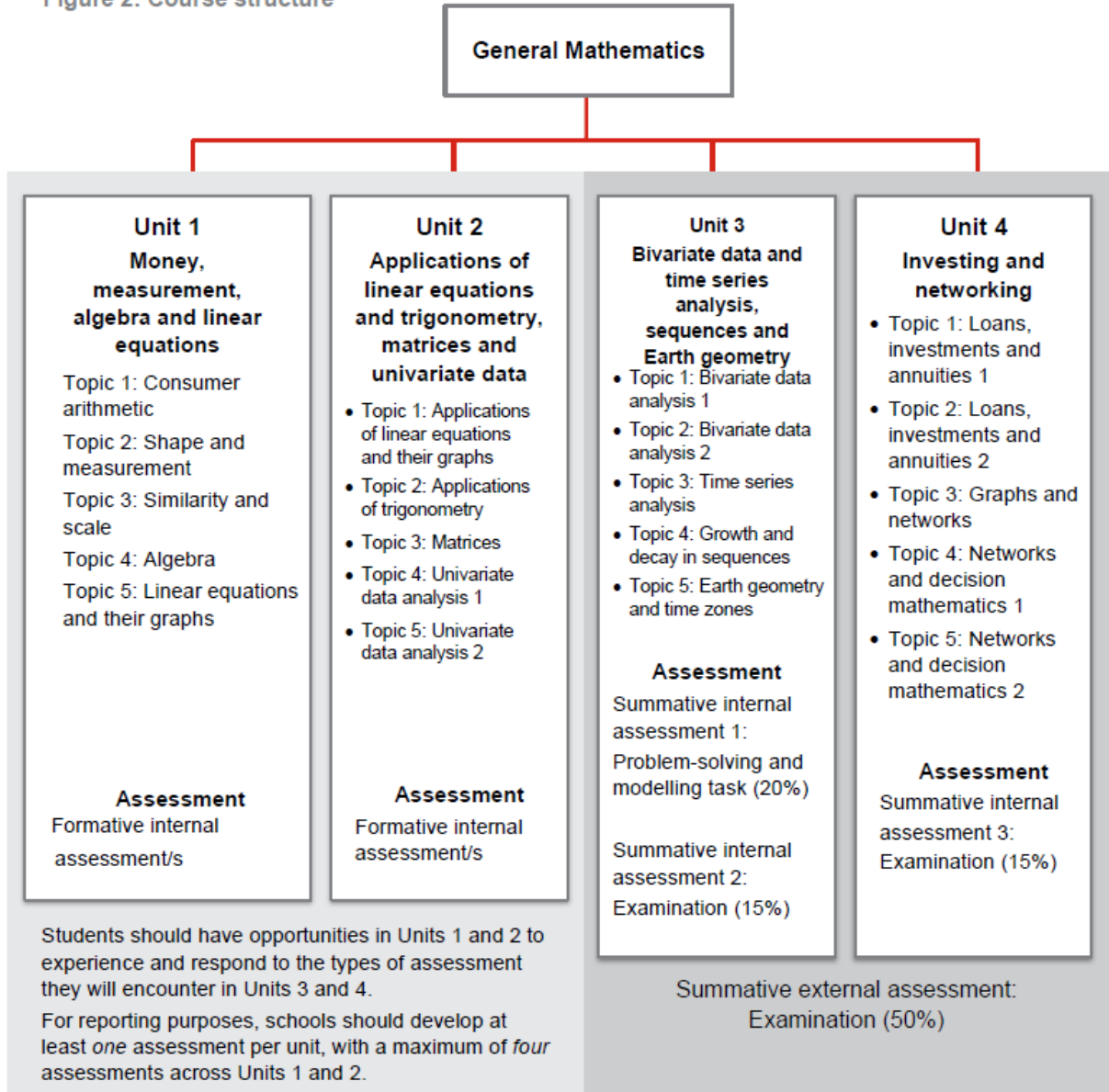
Figure 2: Course structure
