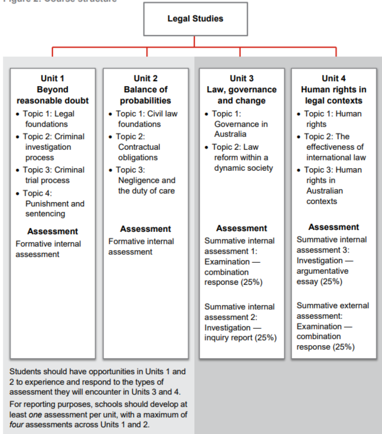
Figure 2: Course structure
