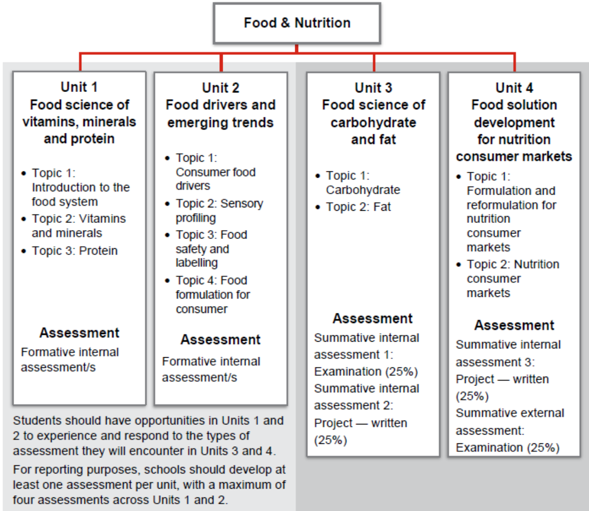
Figure 2: Course structure
