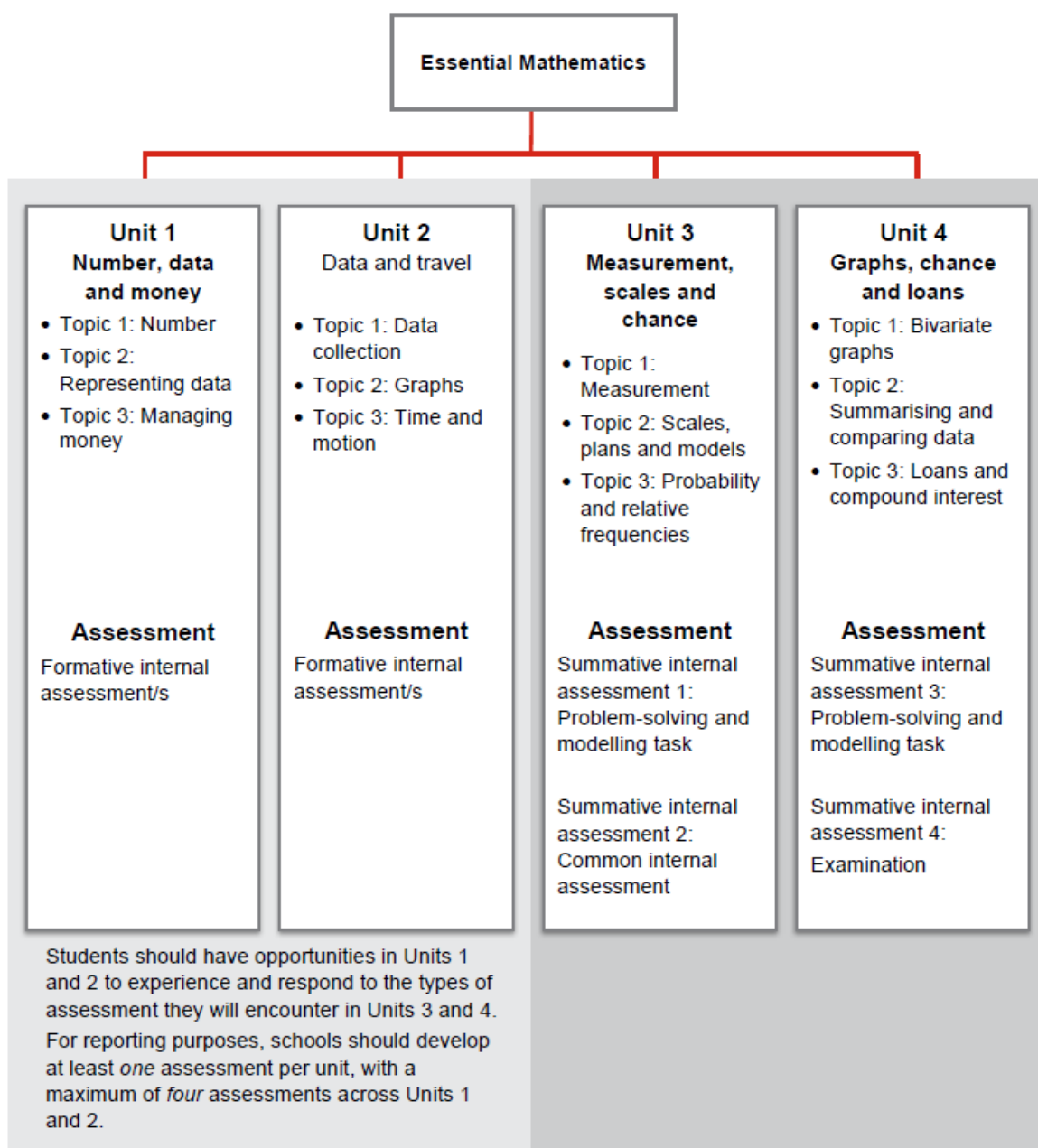
Figure 2: Course structure
